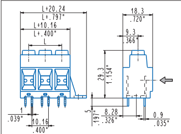
Straight, side stackable, mounting flanges MPS_ZA6-00D 2÷6 poles, 10.16 mm .400" pitch MPSH_ZA6-00D 2÷6 poles, 10.16 mm .400" pitch
