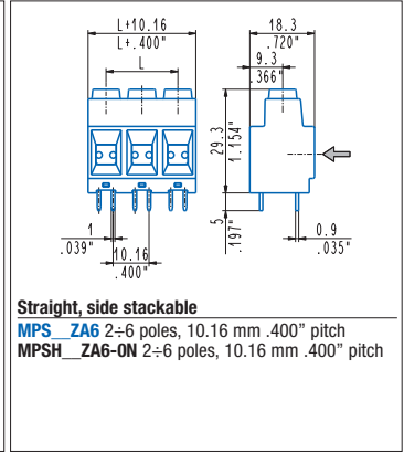
Straight, modular MPS_Z06 2÷6 poles, 10.16 mm .400" pitch MPSH_Z06-ON 2÷6 poles, 10.16 mm .400" pitch
