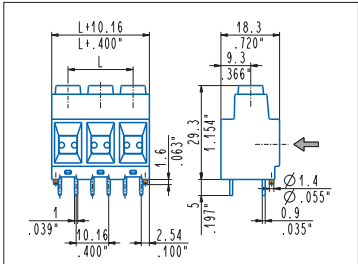
Straight, side stackable, pegs MPS_DA6-0000P 2÷6 poles, 10.16 mm .400" pitch MPSH_DA6-0000P 2÷6 poles, 10.16 mm .400" pitch
