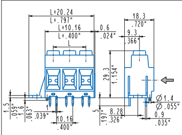
Straight, modular, mounting flanges, peg MPS_Z06-00SOP 2÷6 poles, 10.16 mm .400" pitch MPSH_Z06-00SOP 2÷6 poles, 10.16 mm .400" pitch
