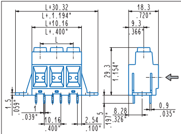
Straight, mounting flanges MPS_DV6 2÷6 poles, 10.16 mm .400" pitch MPSH_DV6-ON 2÷6 poles, 10.16 mm .400" pitch
