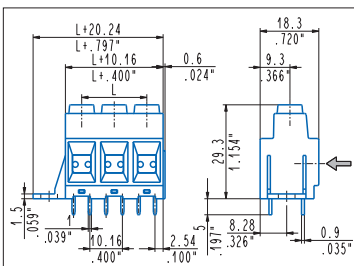
Straight, modular, mounting flanges MPS_D06-00S 1÷6 poles, 10.16 mm .400" pitch MPSH_D06-0NS 1÷6 poles, 10.16 mm .400" pitch
