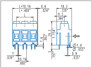
Straight, modular, pegs MPS_Z06-0000P 2÷6 poles, 10.16 mm .400" pitch MPSH_Z06-0000P 2÷6 poles, 10.16 mm .400" pitch
