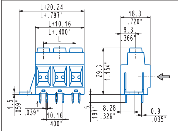
Straight, side stackable, mounting flanges MPS_ZA6-00S 2÷6 poles, 10.16 mm .400" pitch MPSH_ZA6-00S 2÷6 poles, 10.16 mm .400" pitch
