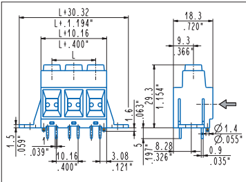
Straight, mounting flanges, pegs MPS_ZV6-0000P 2÷6 poles, 10.16 mm .400" pitch MPSH_ZV6-0000P 2÷6 poles, 10.16 mm .400" pitch
