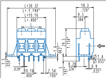
Straight, mounting flanges, pegs MPS_DV6-0000P 1÷6 poles, 10.16 mm .400" pitch MPSH_DV6-0000P 1÷6 poles, 10.16 mm .400" pitch
