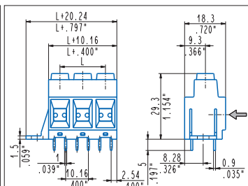
Straight, side stackable, mounting flanges MPS_DA6-00S 1÷6 poles, 10.16 mm .400" pitch MPSH_DA6-0NS 1÷6 poles, 10.16 mm .400" pitch
