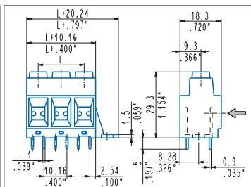
Straight, side stackable, mounting flanges MPS_DA6-00D 1÷6 poles, 10.16 mm .400" pitch MPSH_DA6-0ND 1÷6 poles, 10.16 mm .400" pitch
