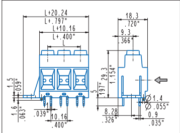
Straight, right mounting flanges, pegs MPS_ZA6-00SOP 2÷6 poles, 10.16 mm .400" pitch MPSH_ZA6-00SOP 2÷6 poles, 10.16 mm .400" pitch
