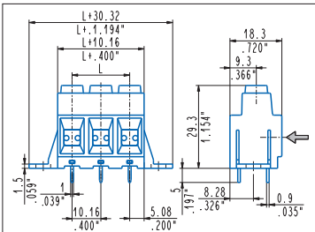
Straight, mounting flanges MPS_SV6 2÷6 poles, 10.16 mm .400" pitch MPSH_SV6-ON 2÷6 poles, 10.16 mm .400" pitch
