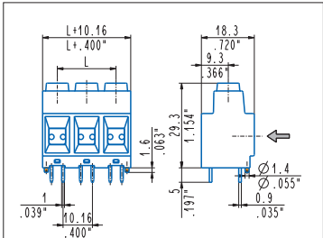
Straight, side stackable, pegs MPS_ZA6-0000P 2÷6 poles, 10.16 mm .400" pitch MPSH_ZA6-0000P 2÷6 poles, 10.16 mm .400" pitch
