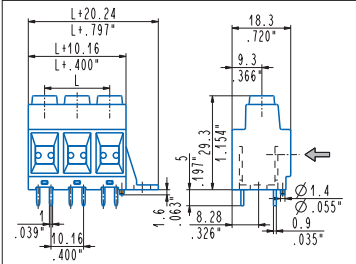
Straight, right mounting flanges, peg MPS_ZA6-00DOP 2÷6 poles, 10.16 mm .400" pitch MPSH_ZA6-00DOP 2÷6 poles, 10.16 mm .400" pitch
