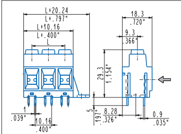
Straight, modular, mounting flanges MPS_Z06-00D 2÷6 poles, 10.16 mm .400" pitch MPSH_Z06-00D 2÷6 poles, 10.16 mm .400" pitch
