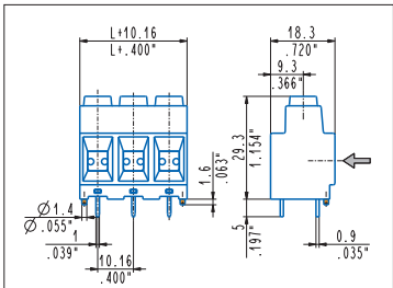
Straight, side stackable, pegs MPS_SA6-0000P 2÷6 poles, 10.16 mm .400" pitch MPSH_SA6-0000P 2÷6 poles, 10.16 mm .400" pitch
