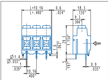
Straight, modular, pegs MPS_S06-0000P 2÷6 poles, 10.16 mm .400" pitch MPSH_S06-0000P 2÷6 poles, 10.16 mm .400" pitch
