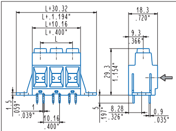
Straight, mounting flanges MPS_ZV6 2÷6 poles, 10.16 mm .400" pitch MPSH_ZV6-ON 2÷6 poles, 10.16 mm .400" pitch
