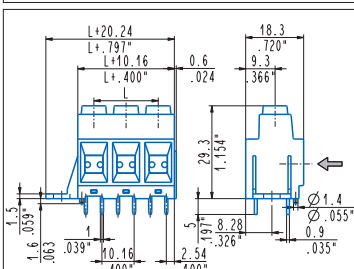
Straight, modular, mounting flanges, peg MPS_D06-00SOP 1÷6 poles, 10.16 mm .400" pitch MPSH_D06-0NSOP 1÷6 poles, 10.16 mm .400" pitch
