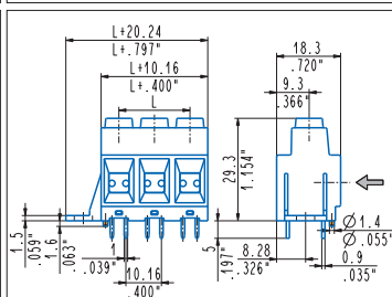
Straight, right mounting flanges, peg MPS_DA6-00SOP 1÷6 poles, 10.16 mm .400" pitch MPSH_DA6-0NSOP 1÷6 poles, 10.16 mm .400" pitch
