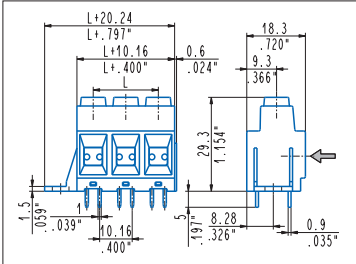
Straight, modular, mounting flanges MPS_Z06-00S 2÷6 poles, 10.16 mm .400" pitch MPSH_Z06-00S 2÷6 poles, 10.16 mm .400" pitch
