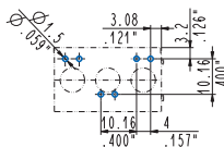
PCB layout "Z" version
