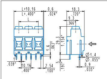
Straight, modular, pegs MPS_D06-0000P 2÷6 poles, 10.16 mm .400" pitch MPSH_D06-0000P 2÷6 poles, 10.16 mm .400" pitch
