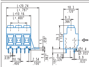
Straight, right mounting flanges, peg MPS_DA6-00DOP 1÷6 poles, 10.16 mm .400" pitch MPSH_DA6-0NDOP 1÷6 poles, 10.16 mm .400" pitch
