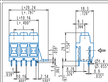
Straight, modular, mounting flanges, peg MPS_D06-00DOP 1÷6 poles, 10.16 mm .400" pitch MPSH_D06-0NDOP 1÷6 poles, 10.16 mm .400" pitch
