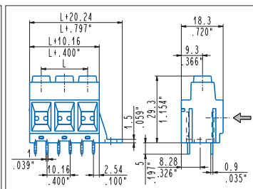
Straight, modular, mounting flanges MPS_D06-00D 1÷6 poles, 10.16 mm .400" pitch MPSH_D06-0ND 1÷6 poles, 10.16 mm .400" pitch
