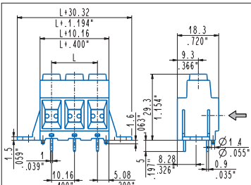
Straight, mounting flanges, pegs MPS_SV6-0000P 2÷6 poles, 10.16 mm .400" pitch MPSH_SV6-0000P 2÷6 poles, 10.16 mm .400" pitch
