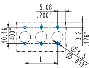
PCB layout "S" version
