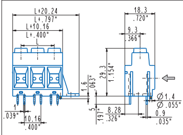
Straight, modular, mounting flanges, peg MPS_Z06-00DOP 2÷6 poles, 10.16 mm .400" pitch MPSH_Z06-00DOP 2÷6 poles, 10.16 mm .400" pitch
